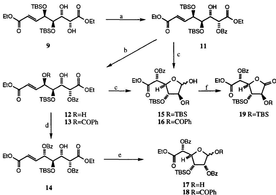
Scheme 2 a) \text{PhCOCl}/\text{Pyr} , b) HF, c) \text{O}_3/\text{DMS} , d) \text{PhCOCl}/\text{Pyr} , e) \text{O}_3/\text{DMS} , f) PCC
