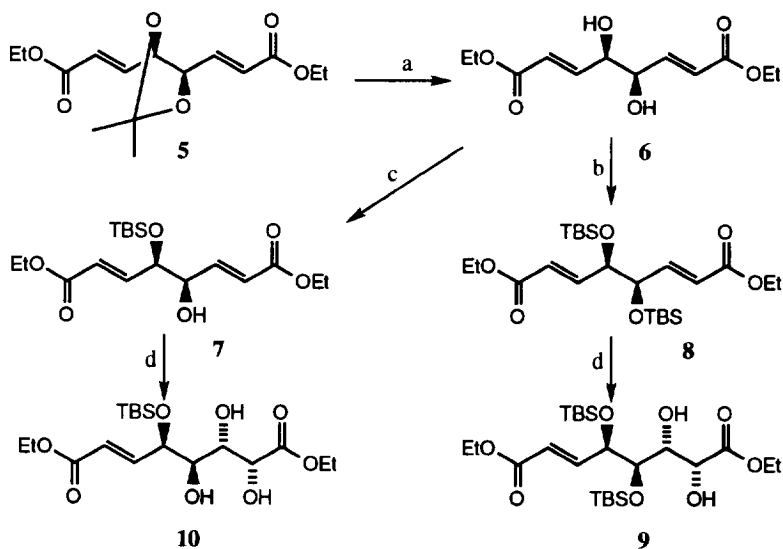
Scheme 1 a) (CH 2 SH) 2 ,BF 3 .OEt 2 . b) 2.4 equiv. TBSCl, imidazole. c) 1.2 equiv. TBSCl, imidazole. d) Cat. OsO 4 , NMO
